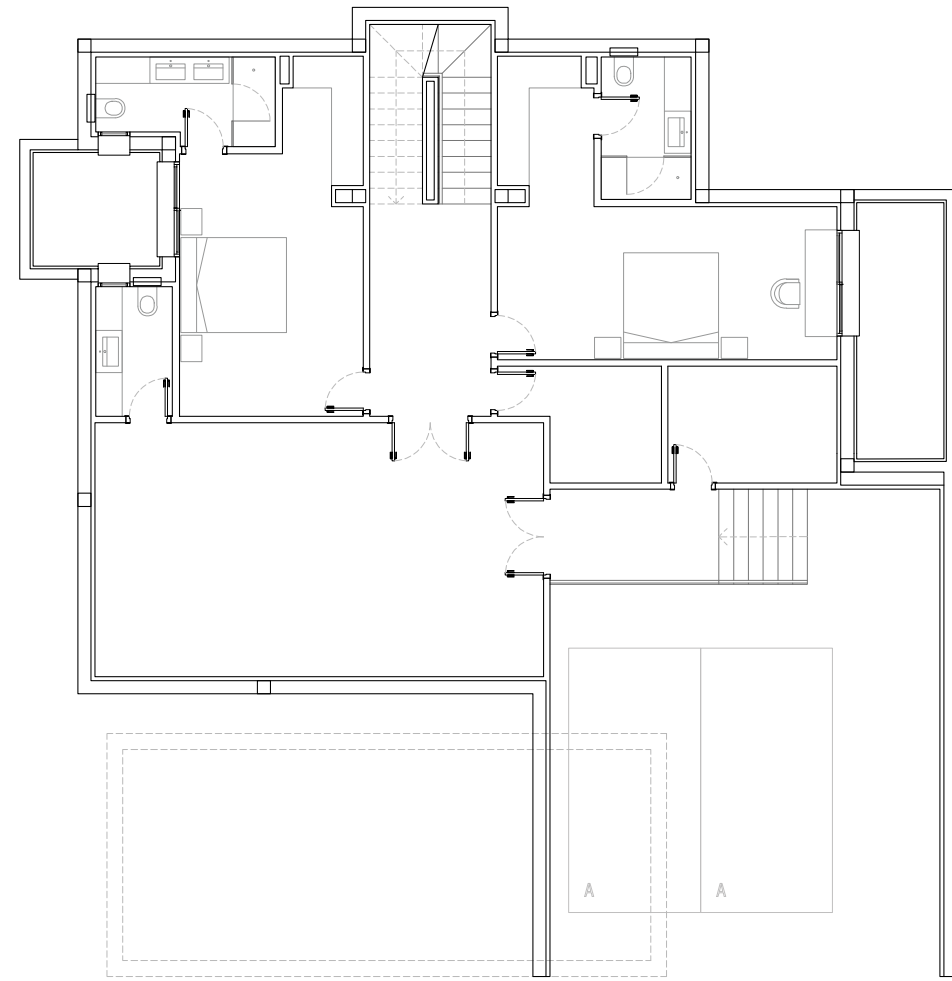
BASEMENT
