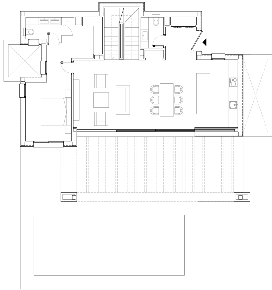
GROUND FLOOR
